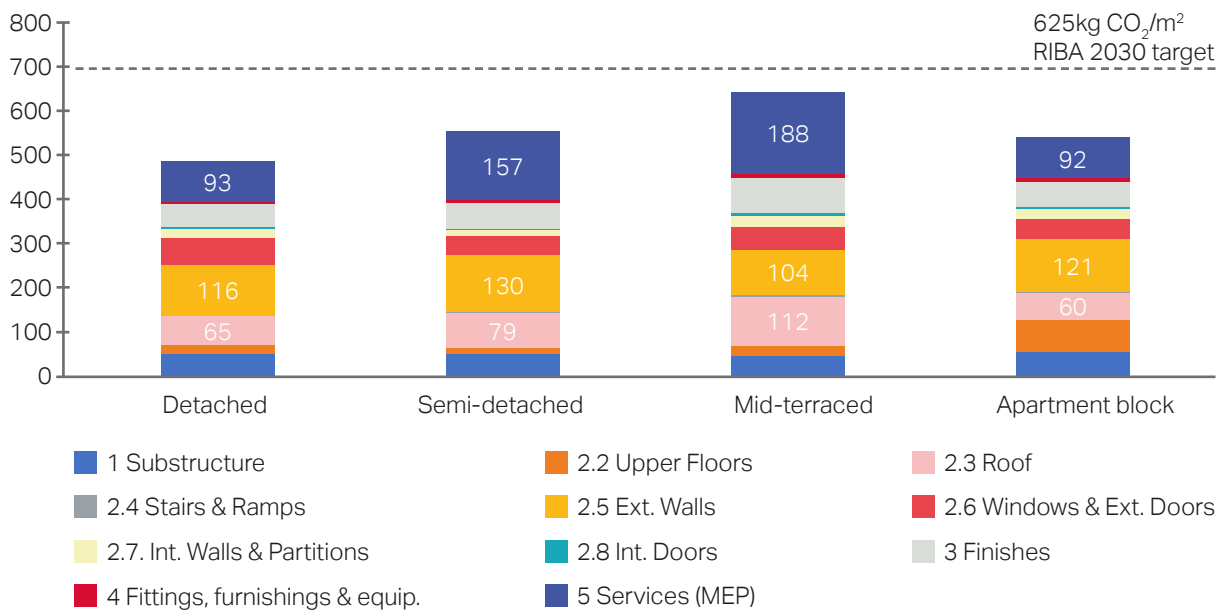
Figure 2 Summary of results of the total embodied carbon for the chosen option of the different dwelling types. Visualisations are indicative only
