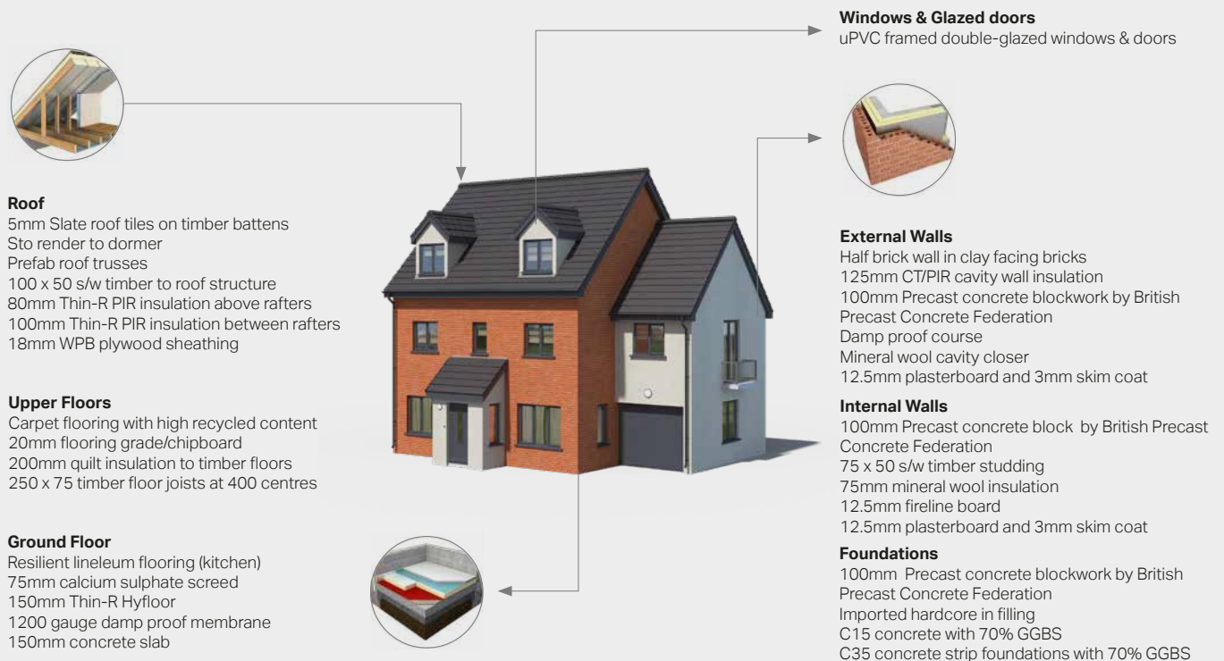
Figure 7 Improved specification of Detached house type
